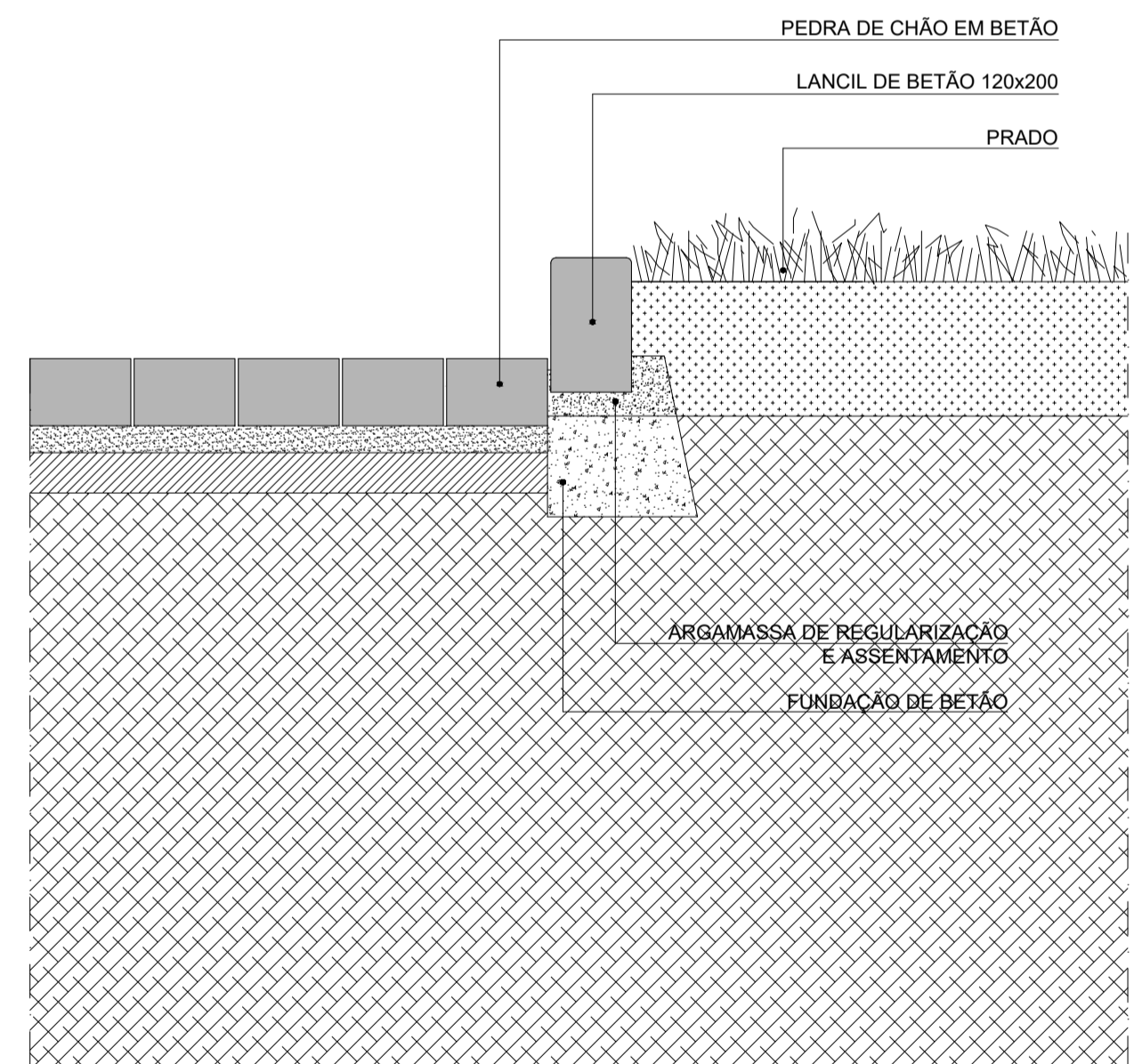
PORMENOR P03
