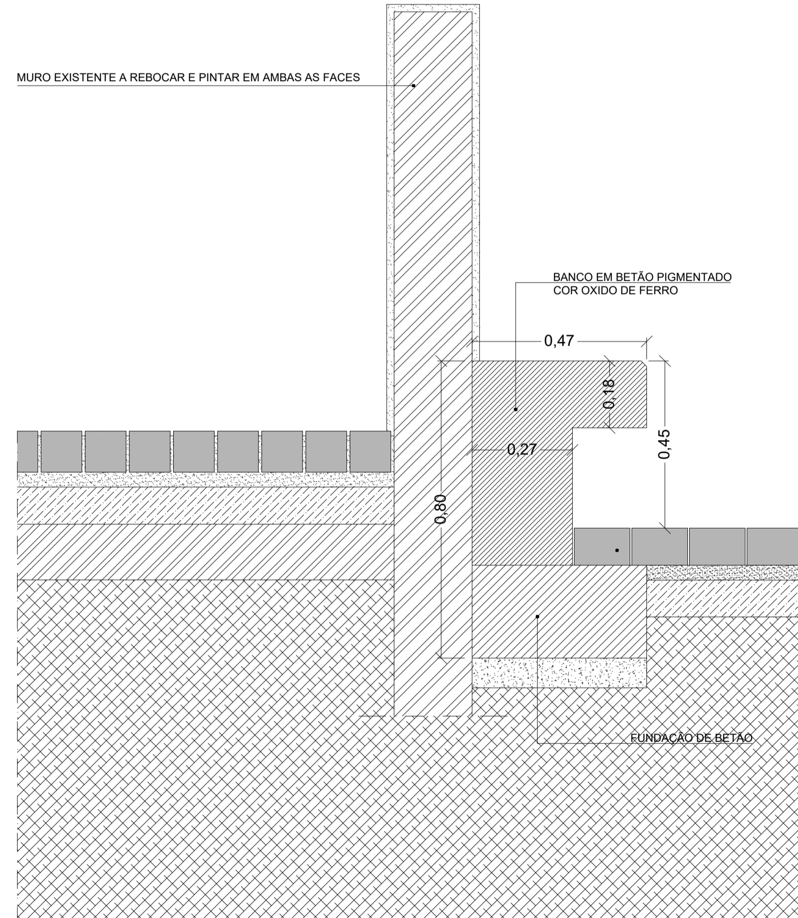
PORMENOR P01
